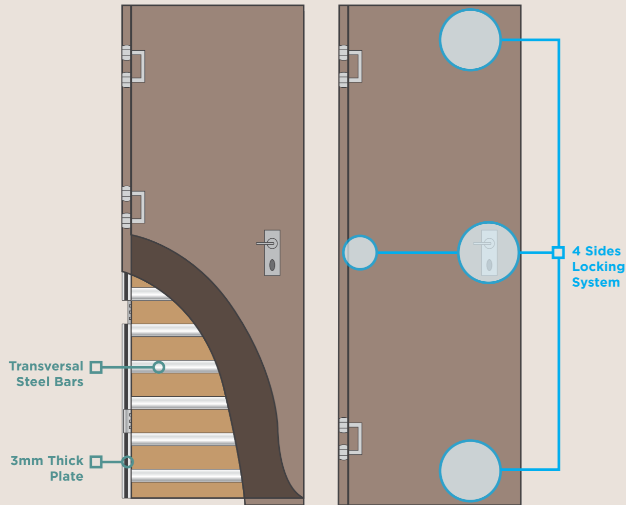
Figure 45: 15 minutes forced entry resistant door
