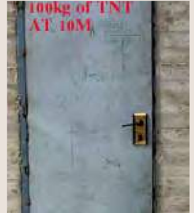
Figure 43: Blast resistant door after a 100kg explosion at 10m
